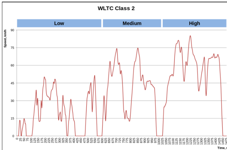
Figure 5: WLTC Class 2 test cycle
