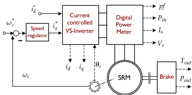
Fig. 6. SyncRel drive and measurement set-up.
